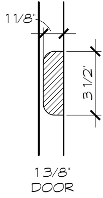
HINGE PREP NOT TO SCALE NOTE: HINGE BACKSET CAN VARY BUT DOOR & FRAME SHOULD BE THE SAME
