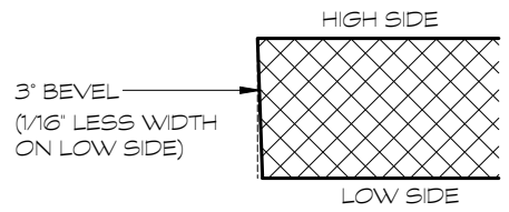
BEVEL DETAIL NOT TO SCALE
